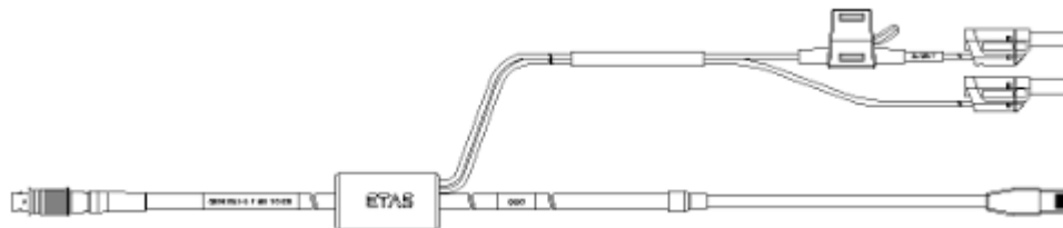
Ethernet PC Connection and Power Supply Cable, Power Feeder close to PC, Lemo 1B FGL - RJ45 - Banana (8fc-8mc+2mc), 5 m
